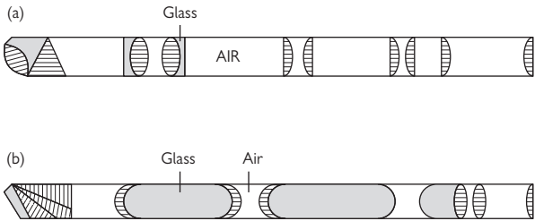
Fig. 17.13 (a) Diagram of conventional cystoscope. The glass lenses are held in place by metal spacers and separated by 'air spaces'; (b) Rod-lens telescope with 'lenses' of air, separated by 'spaces' of glass, with no need for metal spacers. (Reproduced from Blandy J, Fowler C (1995) Urology . Oxford: Blackwell Science, pp. 3–5, with permission from Wiley Blackwell.)
