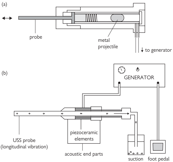
Fig. 9.4 (a) The Lithoclast: a pneumatic lithotripsy device (b) The Calculon: an ultrasonic lithotripsy device. (Reproduced from Walsh PC, Retik AB, Vaughan D, et al. (2002) Campbell's Urology , 8th edn. Amsterdam: W.B. Saunders/Elsevier, pp. 3395–7 with permission from Elsevier).
