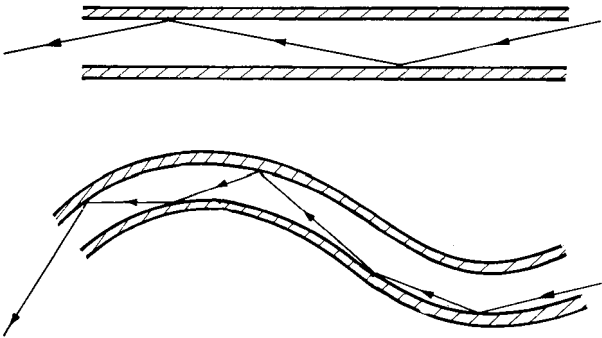
Fig. 17.14 Total internal reflection permits light to travel along a flexible glass fibre. (From Blandy and Fowler 1996, reproduced with permission from Wiley Blackwell. 2 )
